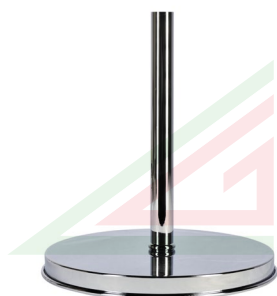
Base cromata Ø 245 mm a 1 sede per asta Ø 22 mm Art. 0301 Ø 245 mm chromed, 1 place for Ø 22 mm pole
