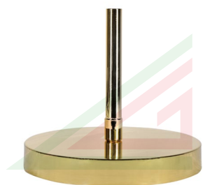
Base ottone Ø 280 mm, 1 sede per asta Ø 22 mm Art. 0321/LUX Ø 280 mm brass, 1 place for Ø 22 mm poles
